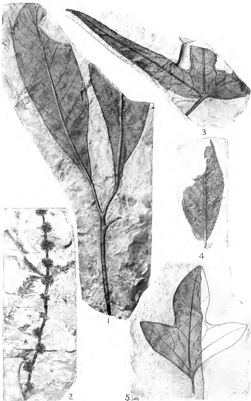
1, Laurus aspensis , new species; 2, Spartanium aspensis , new species; 3, Liquidambar fontuella , new species; 4, Prunus aspensis , new species; 5, Sassafras bradleyi , new species. All natural size.
